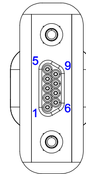
Micro-T
