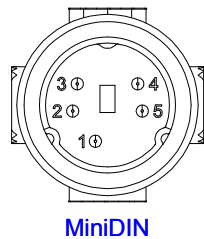
MiniDIN
